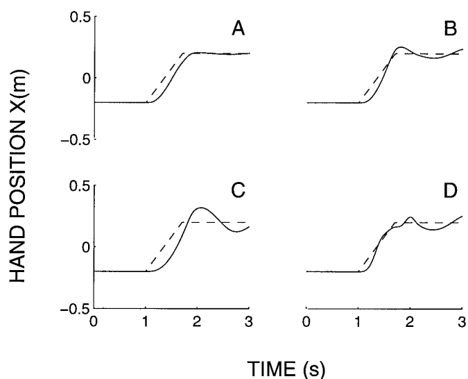
FIG. 8. A : simulated movement comparable with that performed by subjects in the Gomi and Kawato (1996) study. B–D : effects of failing to model a number of physiological properties on the predicted movements. B : effect of removing the velocity dependence of muscle threshold length. In C , the ability to move at different cocontraction levels is eliminated. In D , the dependence of active muscle force on velocity is absent. —, predicted horizontal hand position; - - -, equilibrium hand position over time.
